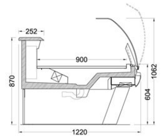
MARINA 122-Y-DC WITH LEGS
