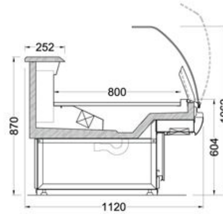
MARINA 112-Y-DC COVERED BASE
