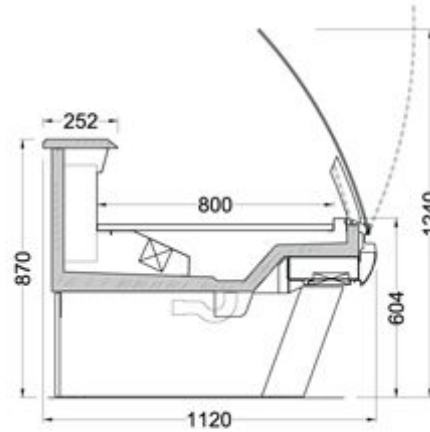
MARINA112-Y-D WITH LEGS
