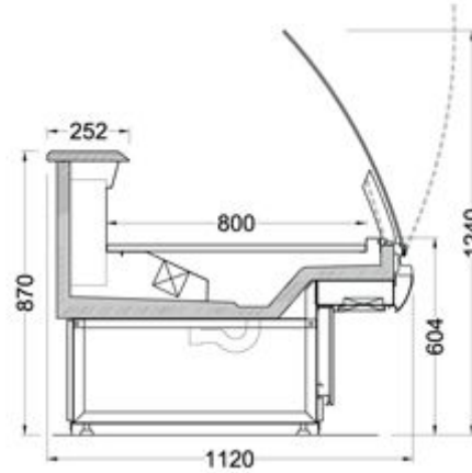
MARINA 112-Y-D COVERED BASE
