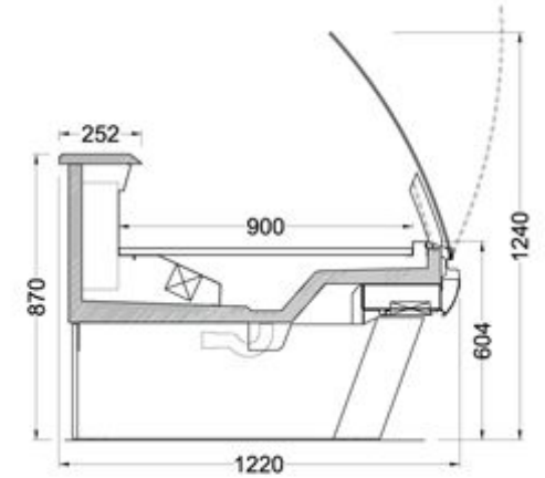
MARINA 122-Y-D WITH LEGS
