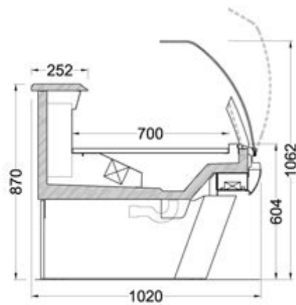
MARINA 102-Y-DC WITH LEGS
