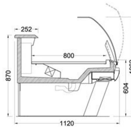
MARINA 112-Y-DC WITH LEGS
