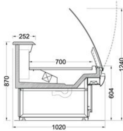
MARINA102-Y-D COVERED BASE
