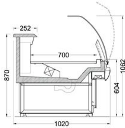
MARINA 102-Y-DC COVERED BASE
