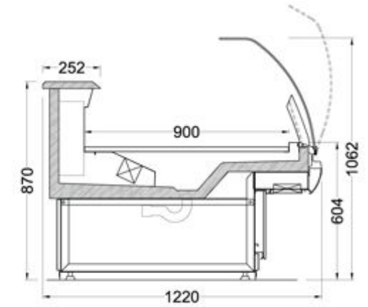
MARINA 122-Y-DC COVERED BASE
