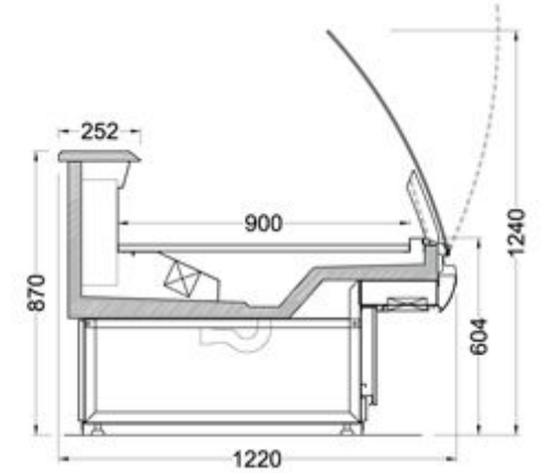
MARINA122-Y-D COVERED BASE
