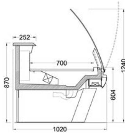
MARINA102-Y-D WITH LEGS
