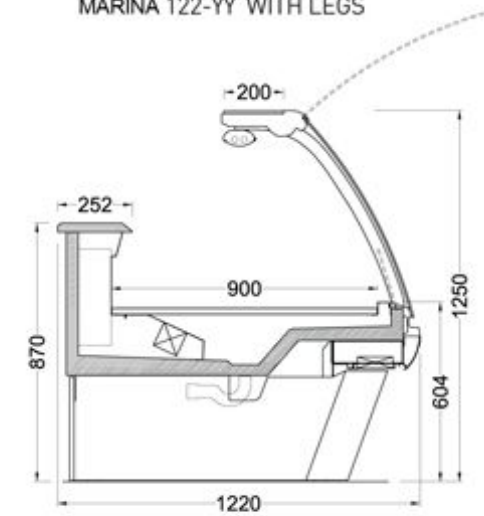
MARINA 122-YY WITH LEGS
