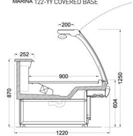
MARINA 122-YY COVERED BASE
