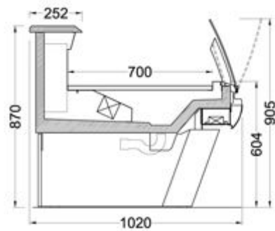
MARINA 102-YY-S WITH LEGS
