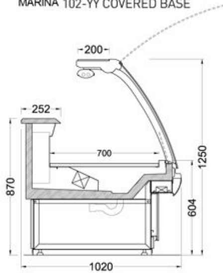
MARINA 102-YY COVERED BASE
