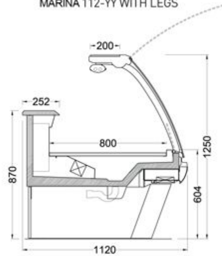
MARINA 112-YY WITH LEGS
