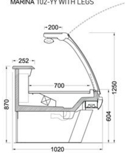
MARINA 102-YY WITH LEGS
