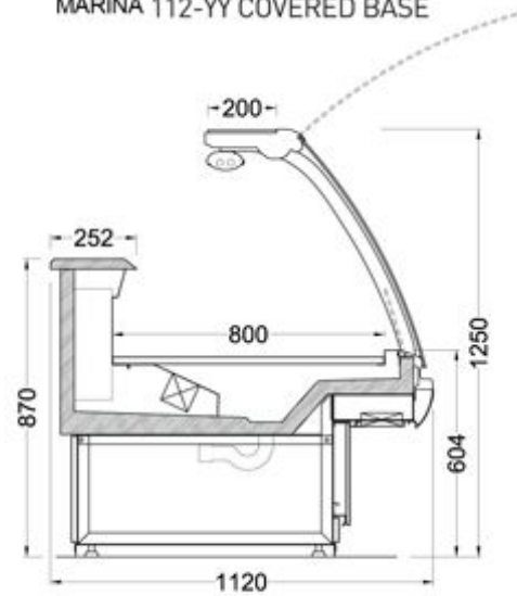
MARINA 112-YY COVERED BASE
