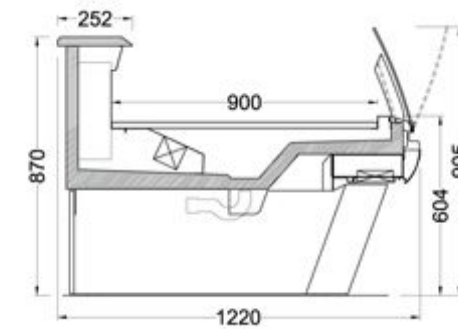
MARINA 122-YY-S WITH LEGS
